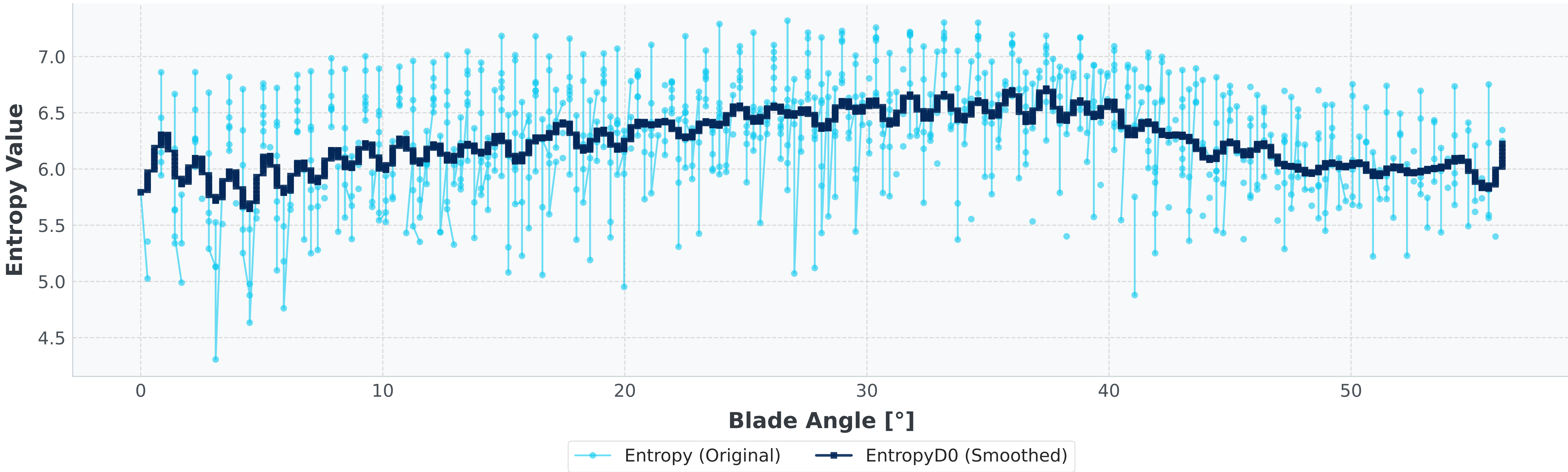
Cloud - Entropy (BLD Phase Averaged)
